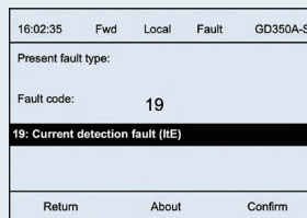
Present fault display interface
