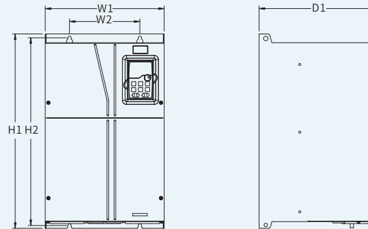
Product outline and mounting dimensions for 380V 090G/110P~110G/132P models
