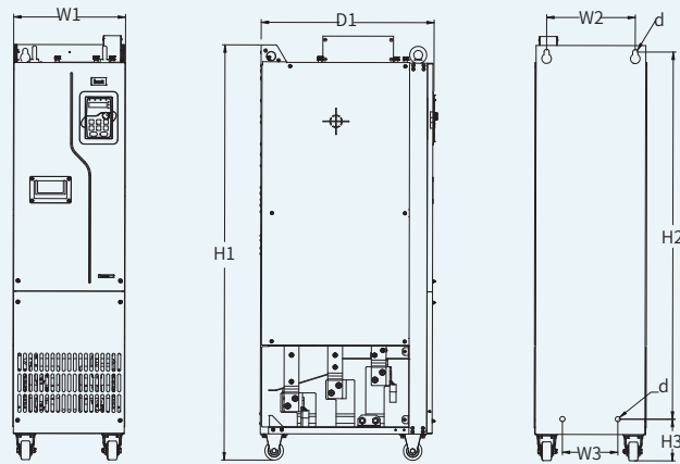
Floor-mounting diagram for 380V 185G/200P-450G/500P models
